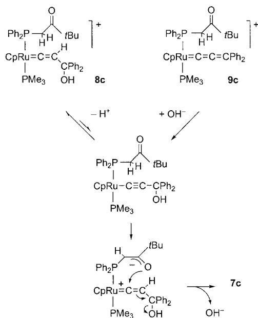
Scheme 3. Rationale accounting (i) for the formation of 7c in methanol and (ii) for the isomerisation of 9c into 7c catalysed by hydroxide anions.
