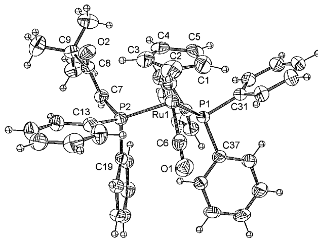
Figure 1. ORTEP drawing of 3b ·CH 2 Cl 2 showing 50% probability thermal ellipsoids. The CH 2 Cl 2 molecule is omitted for clarity. Selected bond lengths [Å] and angles [°]: Ru1–C6 1.858(5), Ru1–P1 2.339(1), Ru1–P2 2.370(1), C7–C8 1.379(5), C8–C9 1.561(6), C8–O2 1.271(5), P2–C7 1.759(4); C7–C8–C9 120.1(4), C7–C8–O2 124.1(4), C8–C7–P2 123.7(3), C9–C8–O2 115.8(4), C7–P2–Ru1 120.7(1), C6–Ru1–P1 90.5(1), C6–Ru1–P2 91.3(1), P1–Ru1–P2 99.19(4).
