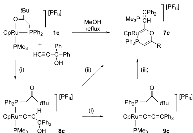
Scheme 2. Reactivity of complex 1c towards 1,1-diphenyl-2-propyn-1-ol: (i) in \text{CH}_2\text{Cl}_2 as solvent, (ii) in MeOH as solvent (room temperature), (iii) in \text{CH}_2\text{Cl}_2 as solvent and in the presence of aqueous \text{K}_2\text{CO}_3 .
