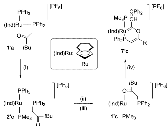
Scheme 4. Synthesis of the new complexes 2'c , 1'c and 7'c : (i) \text{PMe}_3 , \text{CH}_2\text{Cl}_2 , (ii) NaH, THF, reflux, (iii) HCl, \text{NH}_4\text{PF}_6 , MeOH, (iv) \text{HC}\equiv\text{CC}(\text{OH})\text{Ph}_2 , MeOH, reflux.
