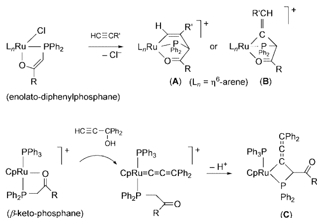
Scheme 1. Carbon–carbon coupling reactions leading to ruthenacycles A–C .
