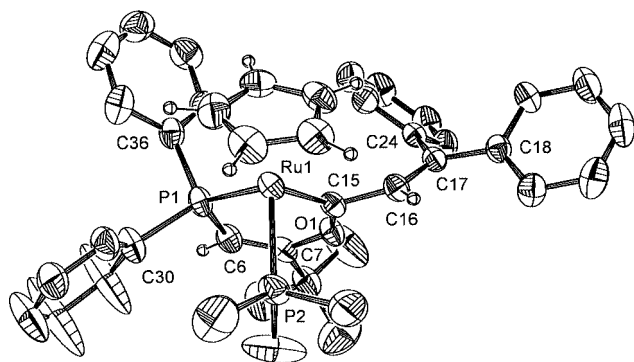
Figure 2. ORTEP drawing of 7c showing 50% probability thermal ellipsoids. The hydrogen atoms and the \text{PF}_6^- anion are omitted for clarity. Selected bond lengths [ \text{\AA} ] and angles [ ^\circ ]: Ru1–C15 1.924(3), Ru1–P1 2.2497(7), Ru1–P2 2.3197(8), C6–C7 1.319(4), C7–O1 1.393(3), P1–C6 1.776(3), C15–C16 1.472(4), C16–C17 1.354(4), C6–P1–Ru1 113.2(1), C7–C6–P1 125.6(2), C6–C7–O1 125.7(3), C7–O1–C15 128.1(2), O1–C15–Ru1 134.3(2), C15–Ru1–P1 90.21(8), C15–Ru1–P2 89.62(8), P1–Ru1–P2 95.57(3), Ru1–C15–C16 119.1(2), C15–C16–C17 129.0(3).
